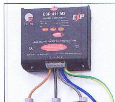
Live connecting leads should be fused accordingly
